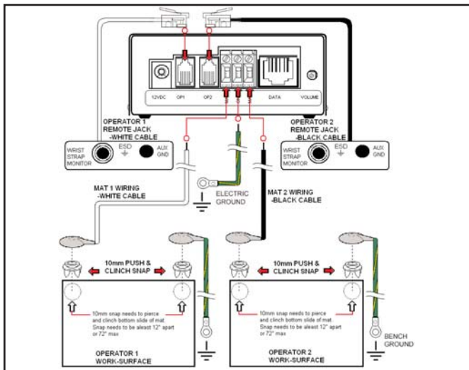
Figure 3. Mat Grounding
