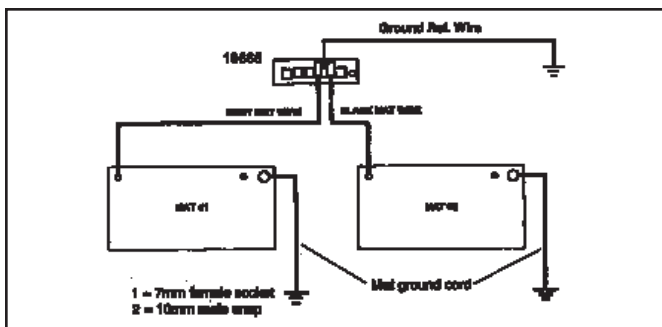
Figure 4. Mat Grounding
