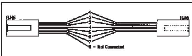
Figure 5. Data Cable
